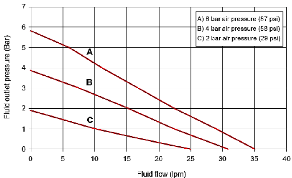
Flow / Pressure
