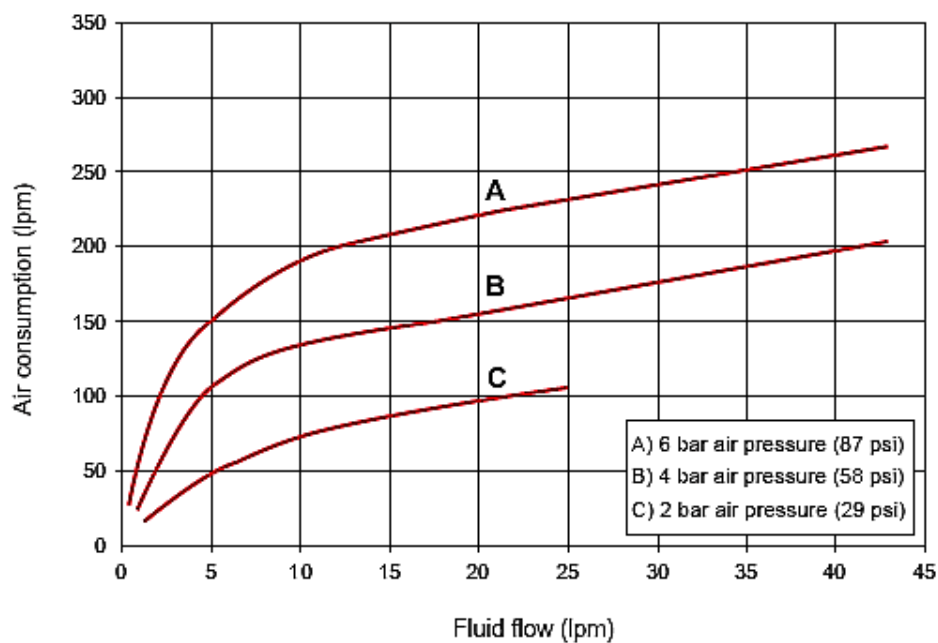
Flow & Air consumption
