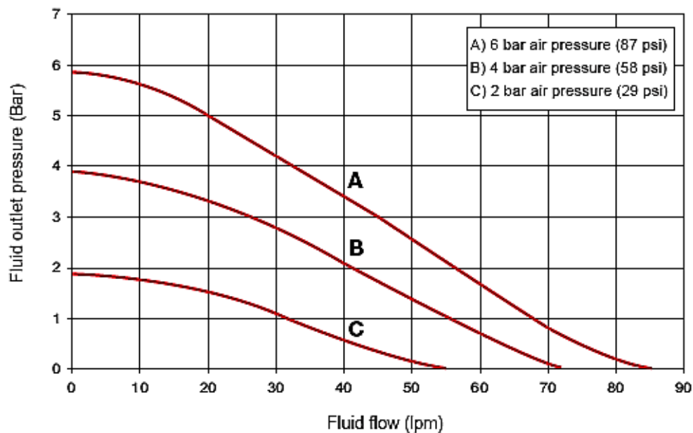
Flow / Pressure
