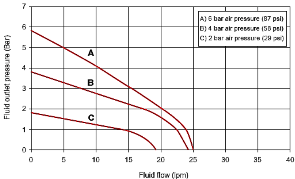
Flow / Pressure
